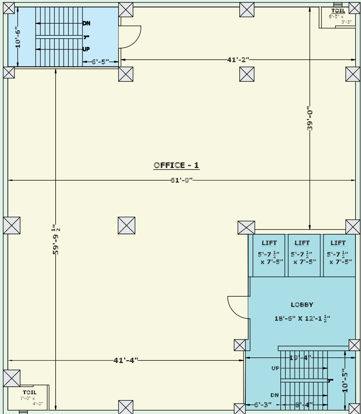
TYPICAL 7TH TO 14TH FLOOR PLAN
